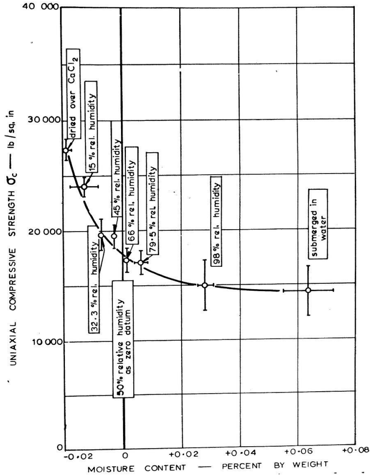
Figure 5. Relationship between uniaxial compressive strength and moisture content for Quartzitic Shale specimens (Colback & Wiid)
