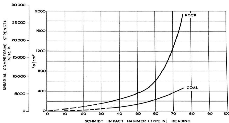
Figure 10. Relationship between the uniaxial compressive strength of rock and the Schmidt impact hammer reading (according to Skutta 61 ).
