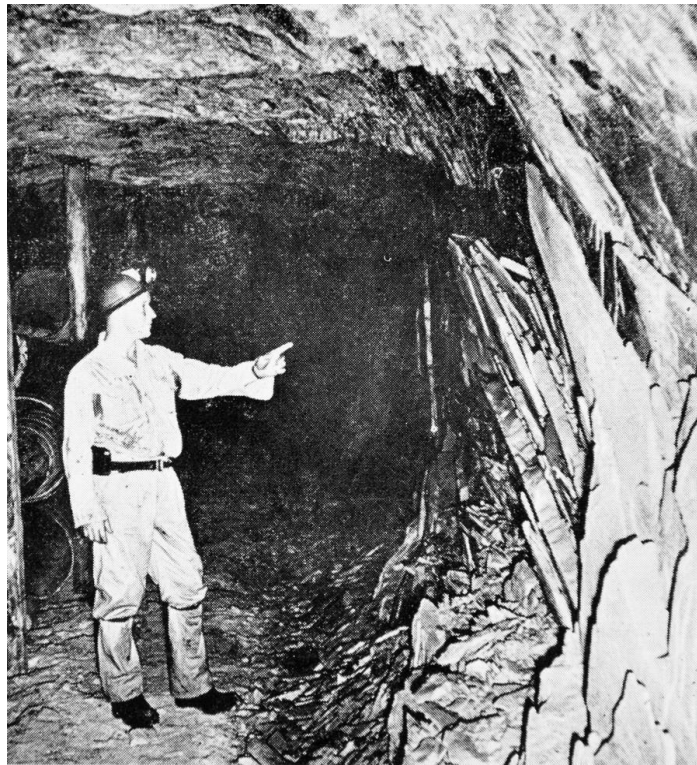
Figure 10b. Sidewall slabbing in a square tunnel in quartzite which had been subjected to a pressure increase due to over-mining. Depth below surface 9,500 ft.
