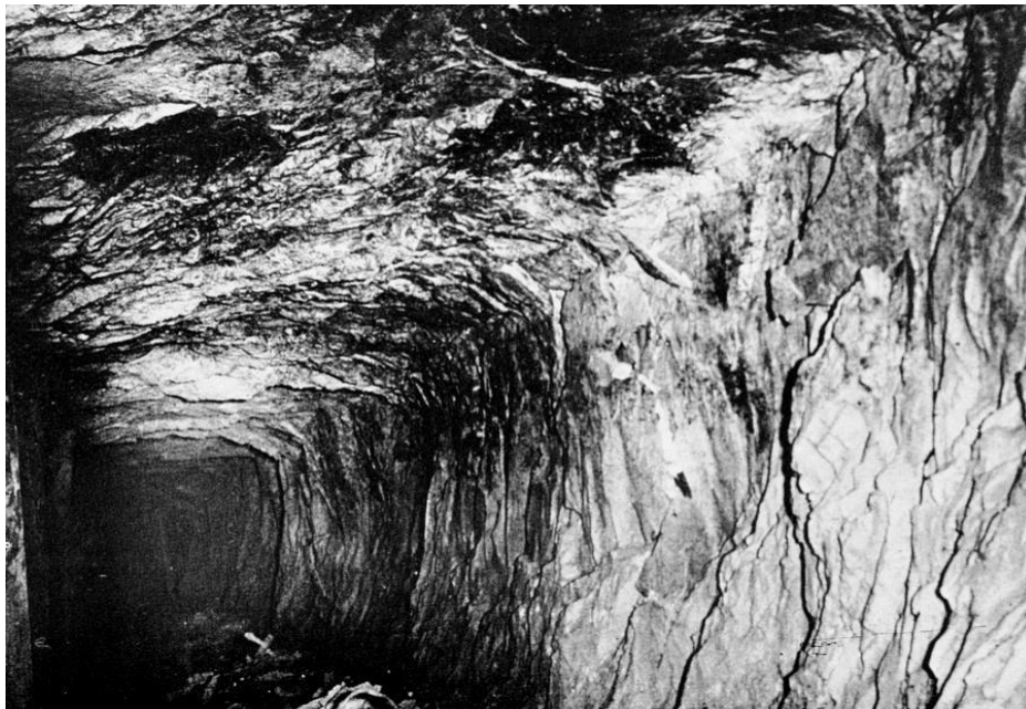
Figure 10a. Square tunnel in quartzite remote from mining activities. Depth of 9,500 ft. below surface in a South African gold mine
