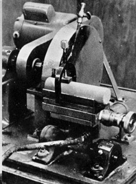
Figure 8: Machine used by the C.S.I.R. for grinding the ends of cylindrical specimens.
