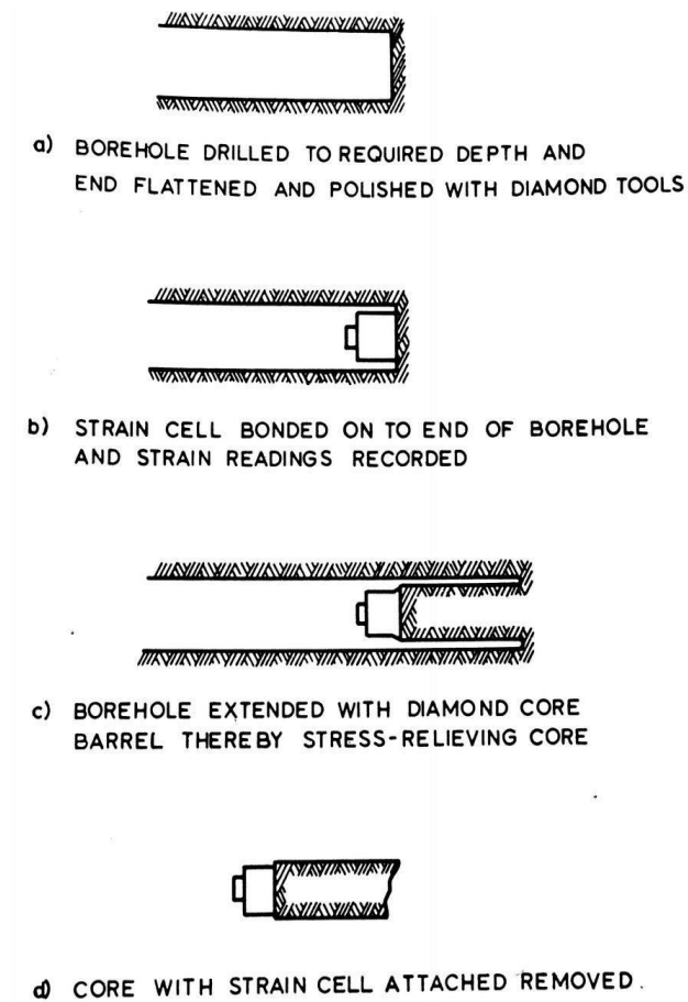
Figure 3. Sequence of operations in Leeman's method for measuring rock stress.
