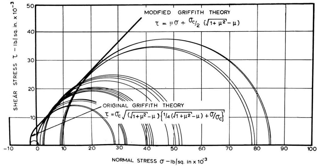
Figure 3. Mohr fracture diagram for typical Witwatersrand quartzite with a uniaxial compressive strength \sigma_c = 30,000 p.s.i. and a coefficient of internal friction \mu = 1.00 .
