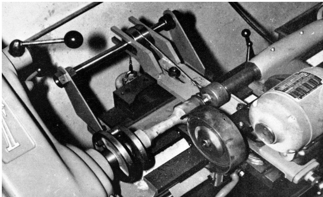
Figure 9. Preparation of tensile specimens using a diamond impregnated grinding wheel mounted on a toolpost grinder on a lathe.
