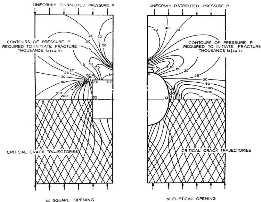
Figure 8. Fracture contours and critical crack trajectories in quartzite surrounding square and elliptical tunnels
