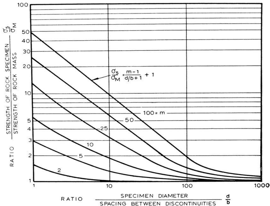
Figure 7. Relationship between specimen size and strength according to Protodiakonov
