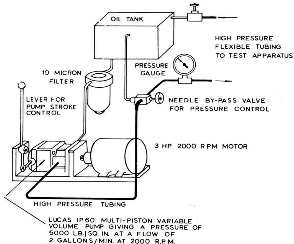
Figure 11. Circuit used for producing accurately controlled hydraulic pressures.
