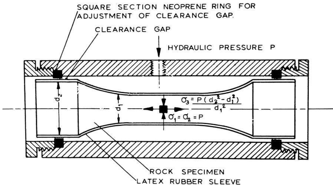
Figure 12. Apparatus for determining the tensile strength of rock specimens.
