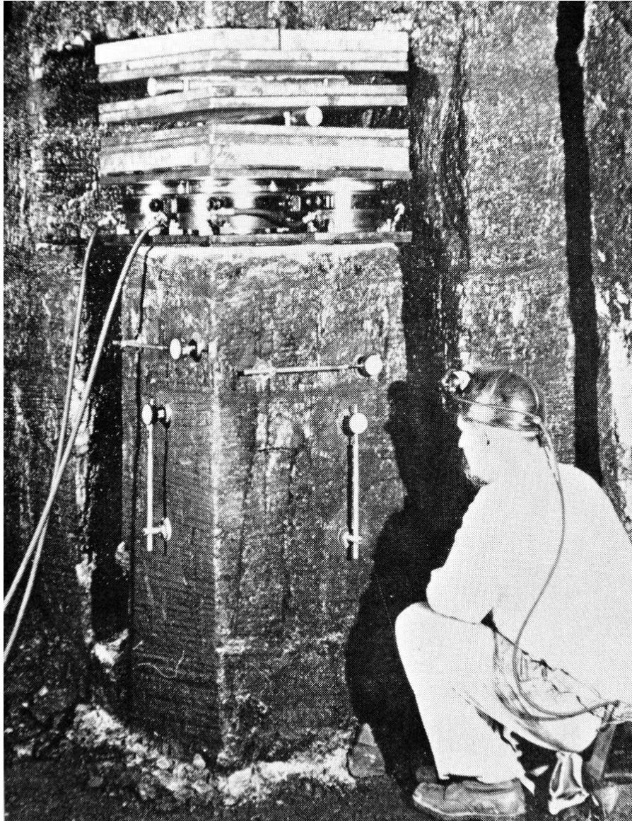
Figure 9. A large scale coal specimen under test.
