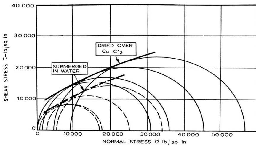
Figure 6. Mohr fracture envelopes showing the effect of moisture on the compressive strength of quartzitic shale (from Colback & Wiid)
