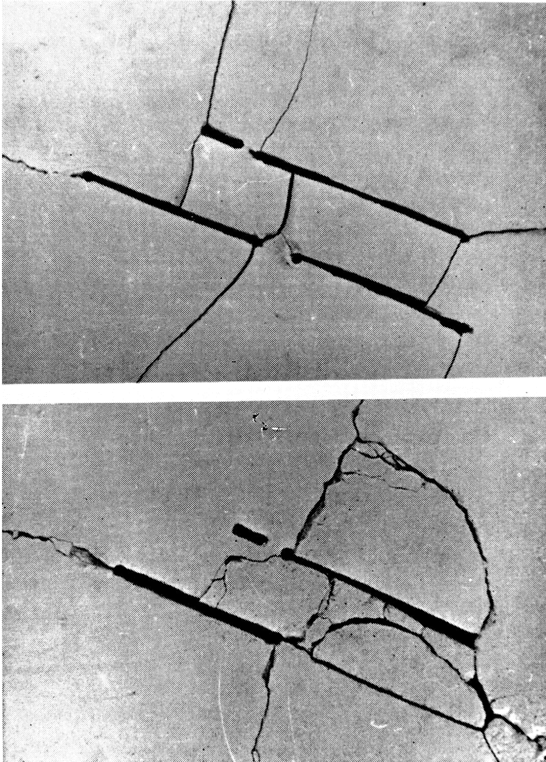
Figure 16. Comparison between the propagation of fracture in plaster of Paris models subjected to uniformly distributed edge loading (upper photograph) and centrifugal loading (lower photograph).
