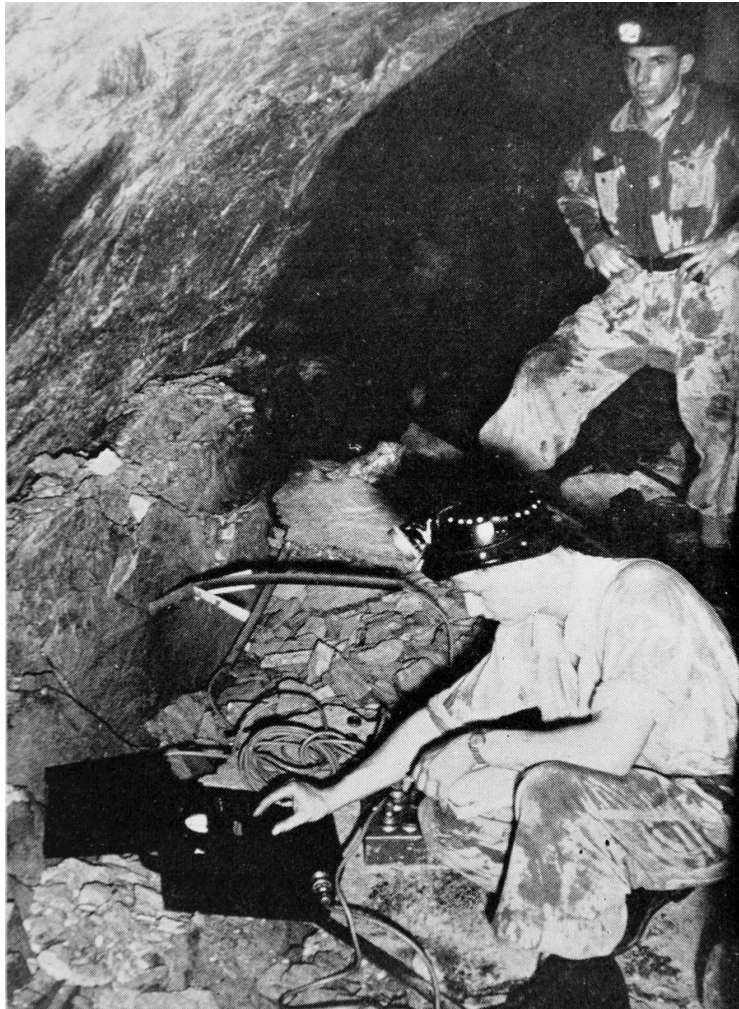
Figure 4. The measurement of stress in a deep level South African gold mine.
