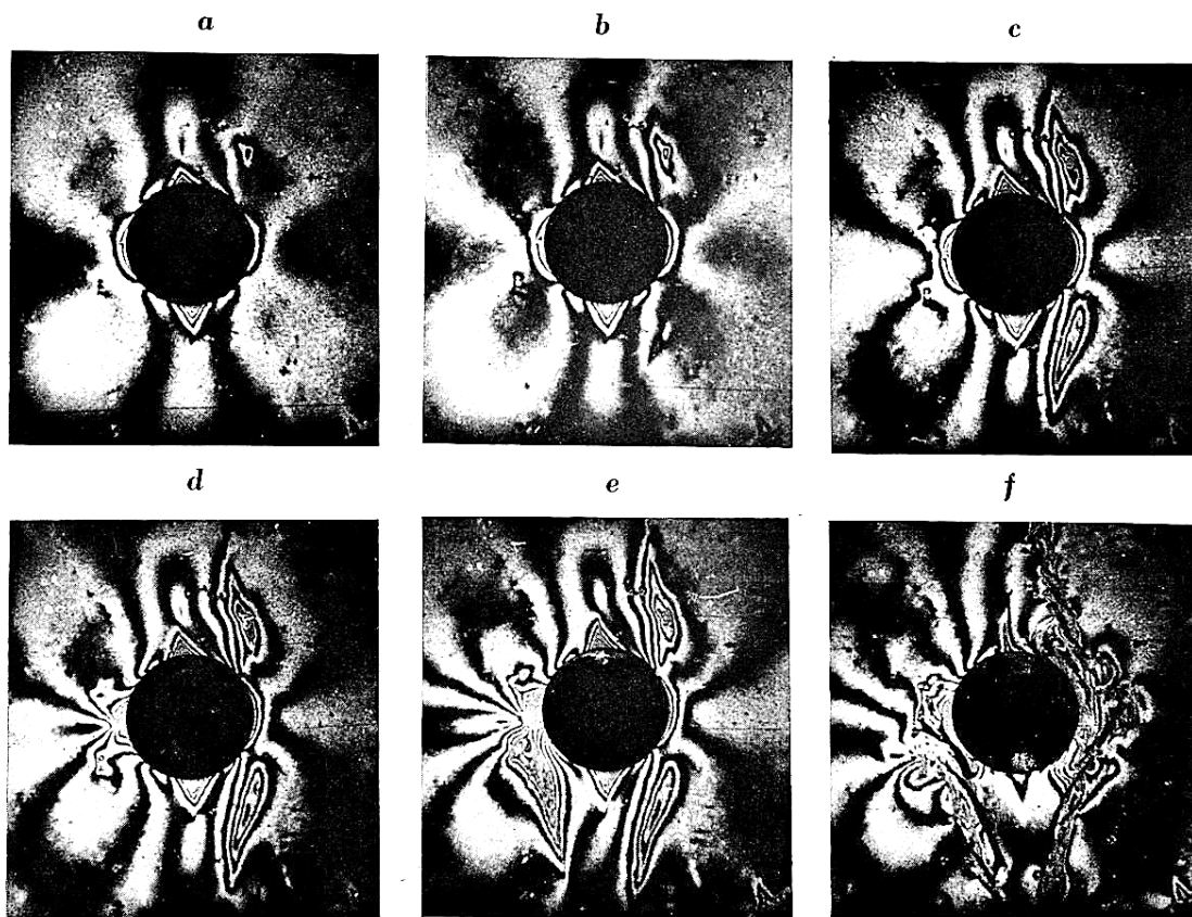
Figure 15. Reflected light photographs of the photoelastic patterns induced in a birefringent lay by fracturing of the rock surrounding a circular excavation in a plate model.
