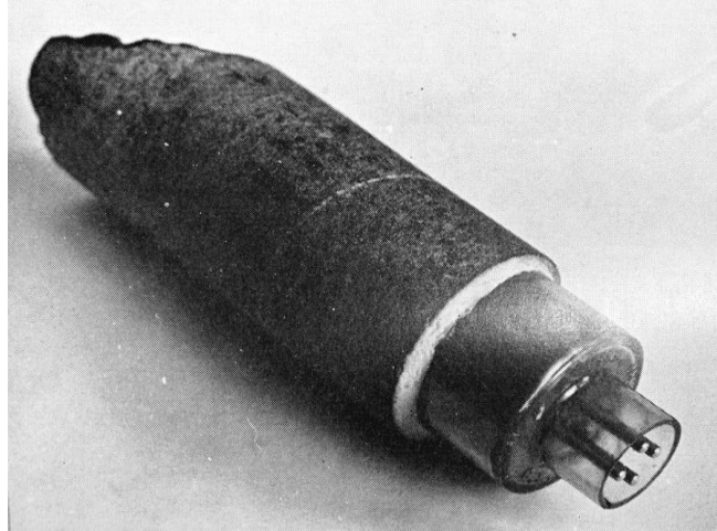
Figure 2. A C.S.I.R. Strain cell bonded on to a rock core recovered from a borehole.
