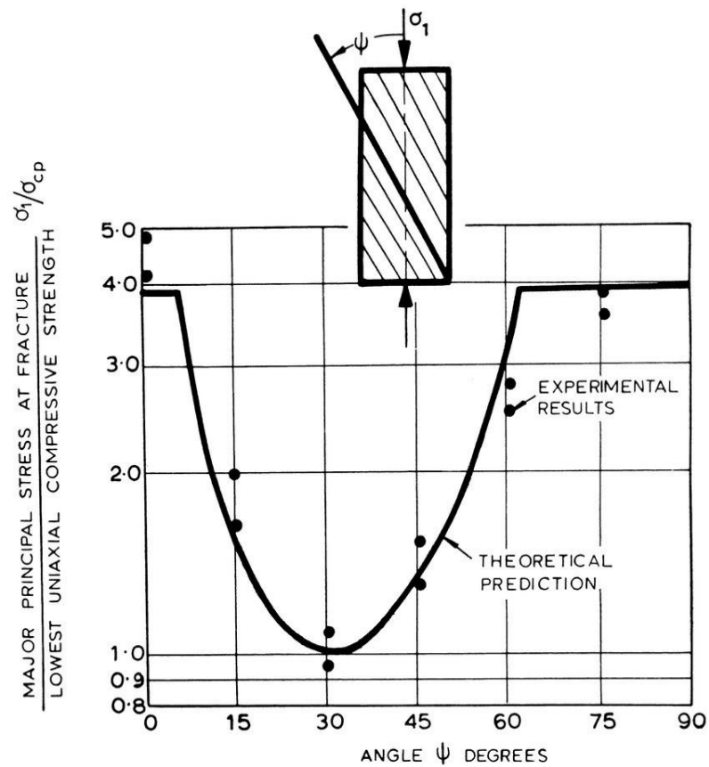
Figure 4. Relationship between bedding plane orientation and strength of slate.
