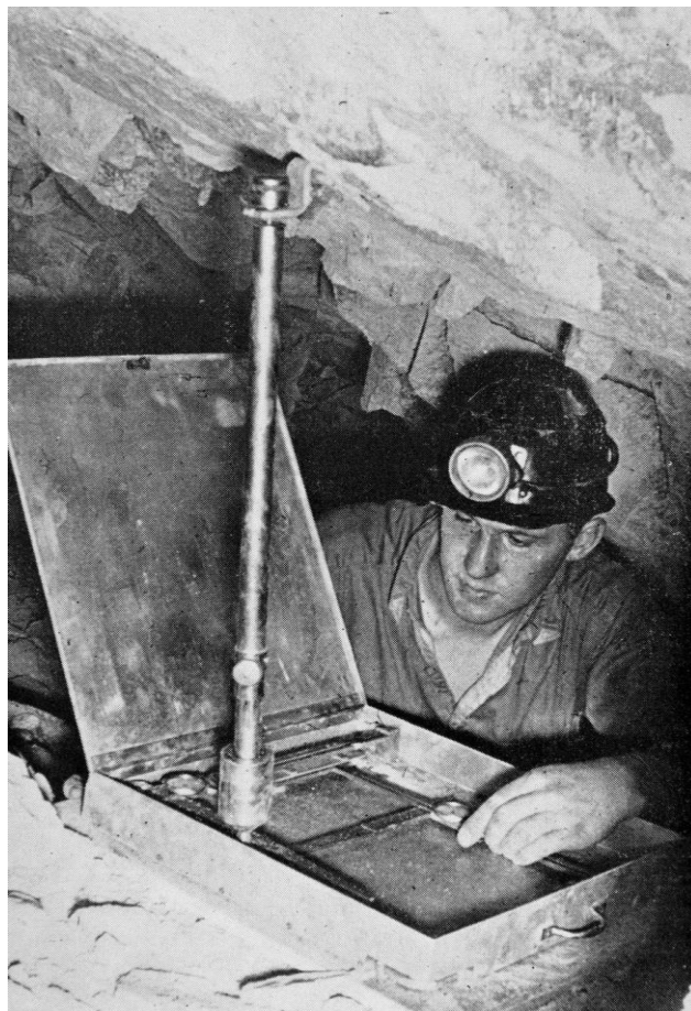
Figure 1. An instrument used by the South African C.S.I.R. for the measurement of closure and ride in a slope in a deep-level gold mine.
