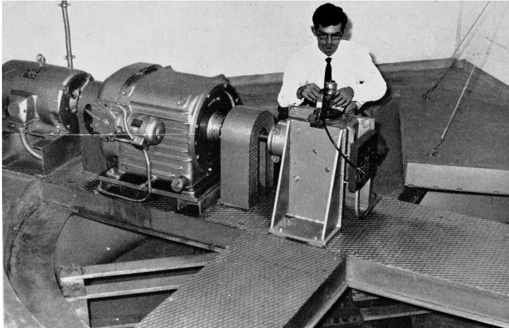
Figure 5. The C.I.S.R.'s 9 ft. diameter centrifuge for subjecting models to acceleration of up to 1,000 times the acceleration due to gravity.
