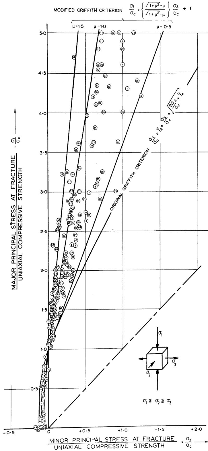
Figure 2. Triaxial fracture data for 50 rock and concrete materials listed in Table 1.
