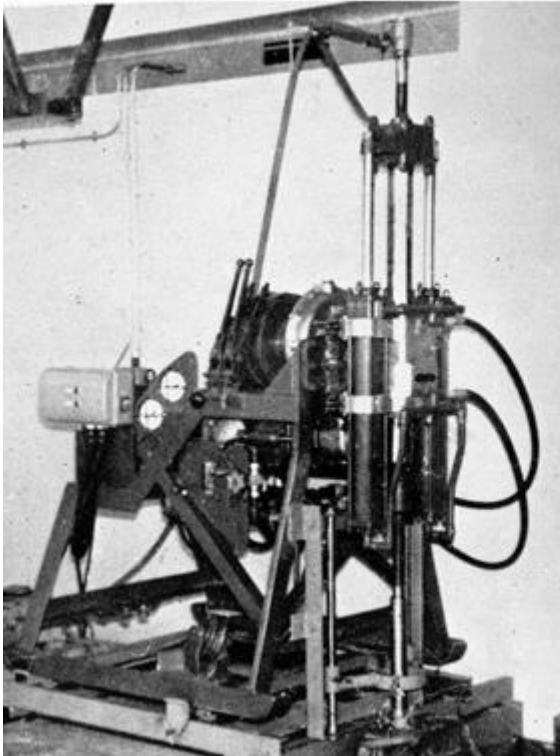
Figure 7: Hydraulically driven diamond drilling machine used for specimen recovery from rock blocks.
