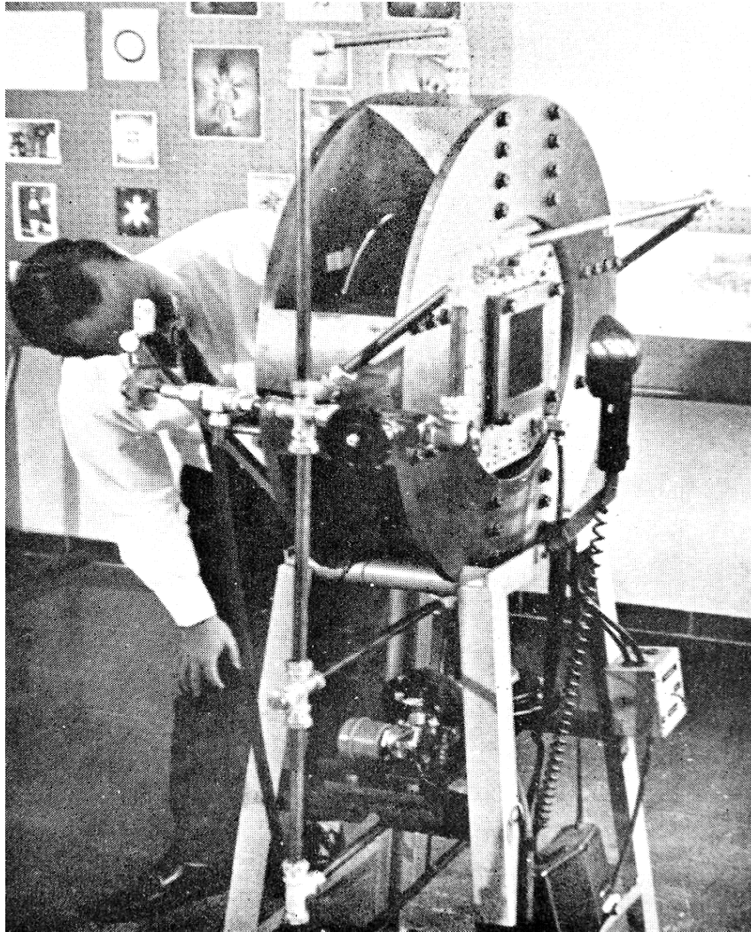
Figure 14. Apparatus used by the C.S.I.R. for subjecting plate models to biaxial compressive loading.
