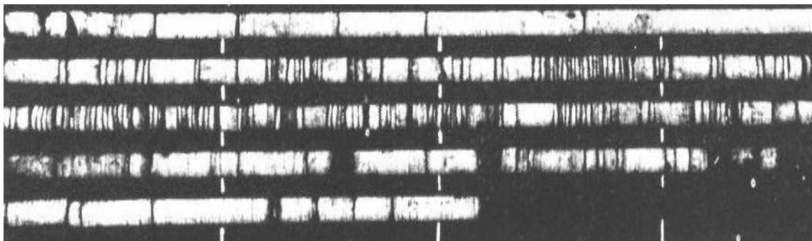
Figure 5. Dinking of core recovered from a borehole drilled into highly stressed rock.
