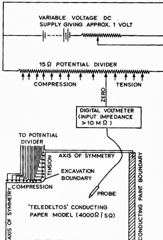
Figure 3. Circuit for conducting paper analogue.
