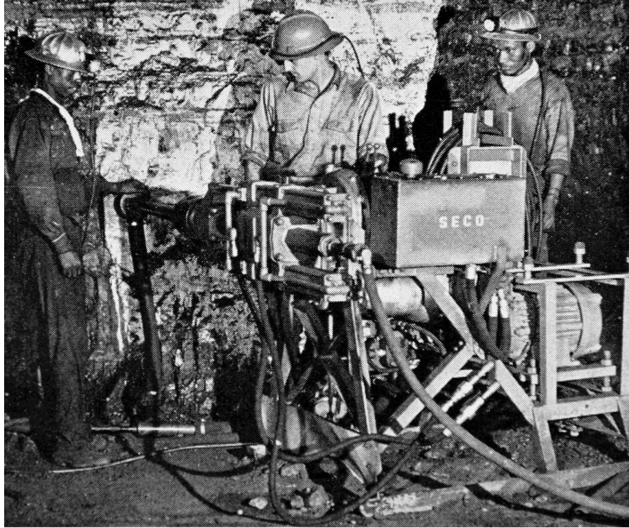
Figure 7. Drilling coal specimens for properties testing
