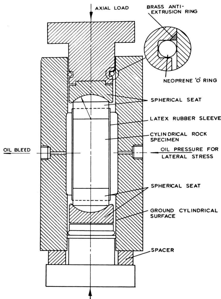
Figure 10. Apparatus for subjecting cylindrical rock specimens to triaxial compressive stress conditions.
