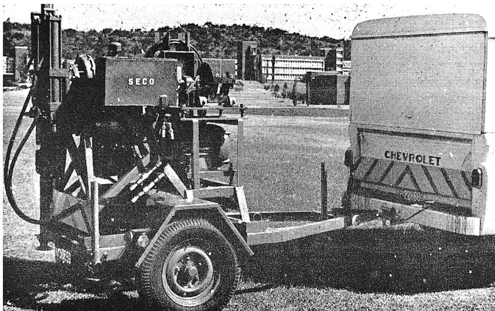
Figure 6. Mobile equipment used by the South African C.S.I.R. for drilling and specimen preparation in coal mines.
