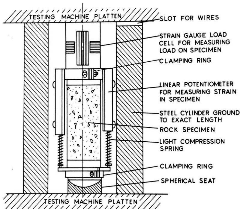
Figure 13. Apparatus for tests to simulate load transfer from a specimen at point of failure.
