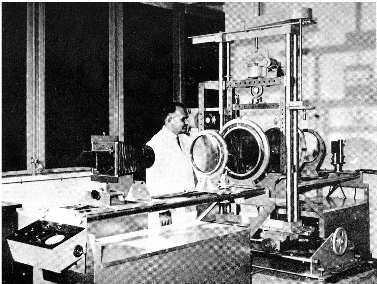
Figure 1. The C.S.I.R. polariscope for producing a 12 in. diameter beam of polarised light for photoelastic model analysis.
